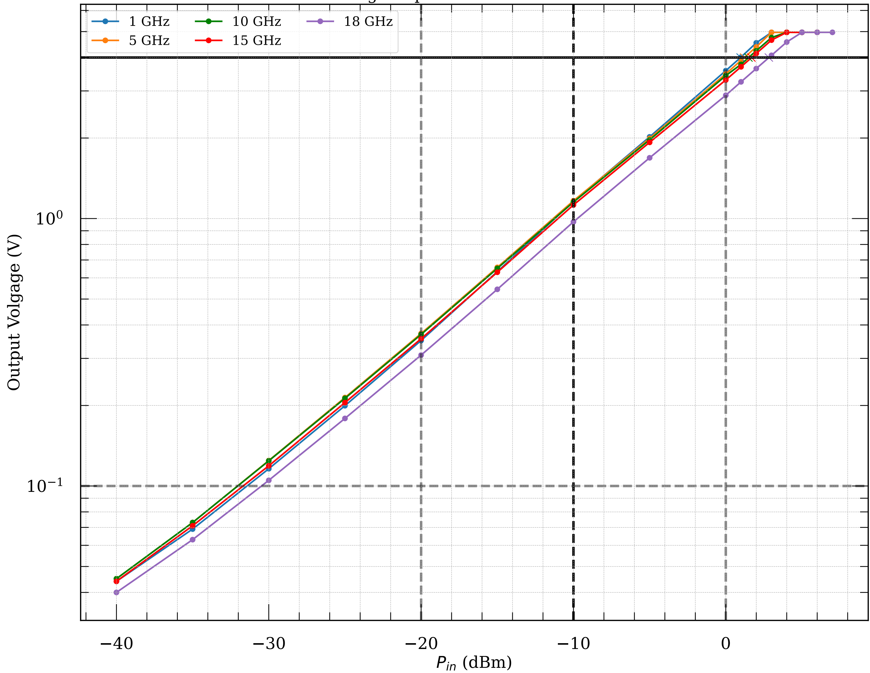
Measured voltage-to-power curve of detector module093
